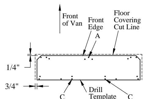
Figure 6: Floor covering cut location (top view).
