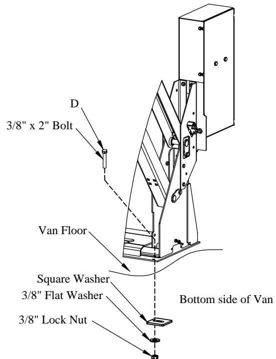
Figure 18: Passenger side "D" location hole and fastener.
