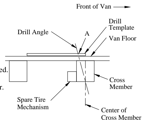
Figure 5: Section Y-Y, side view of "A" drilling location (side view).
