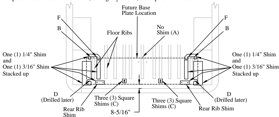
Figure 8: Rib shim locations (top view).
