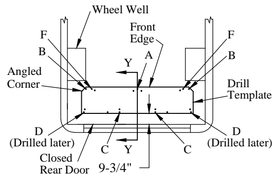
Note: This is not the final location of the liftgate. Figure 4: Drill template location (top view).
