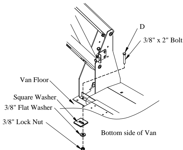
Figure 17: Driver side "D" location hole and fastener.
